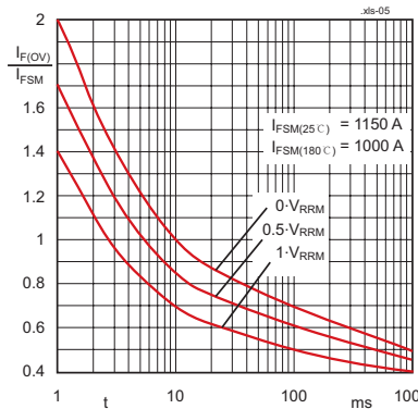
Fig. 6 Surge overload current vs. time
