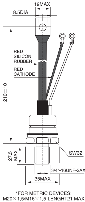
Case Style TO-93(ceramic)
